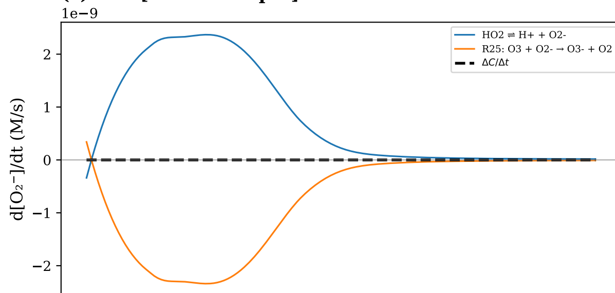
(c) O 2 - [final=1.72 pM]
