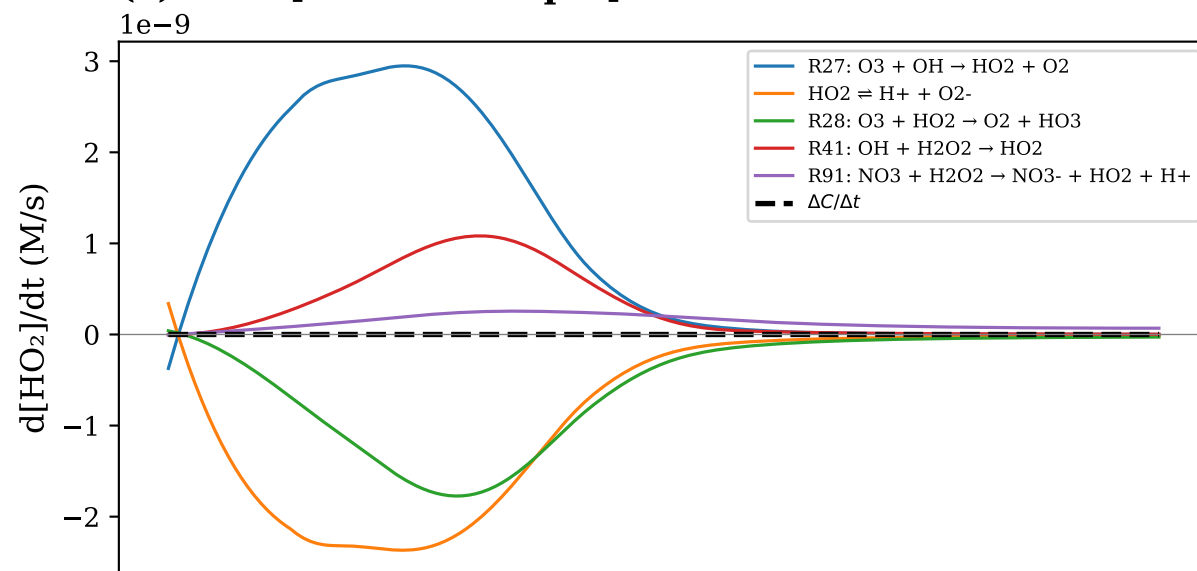
(a) HO 2 [final=12.09 pM]
