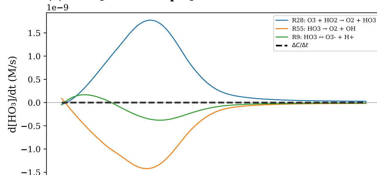
(b) HO 3 [final=0.00 pM]
