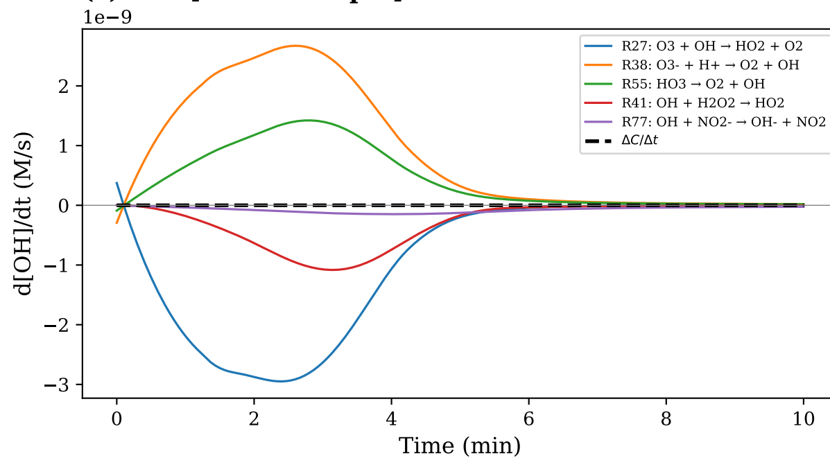
(e) OH [final=0.01 pM]
